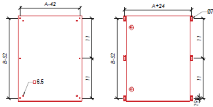
WALL MOUNTING
