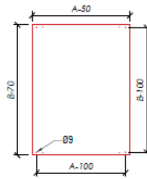
MOUNTING PLATE
