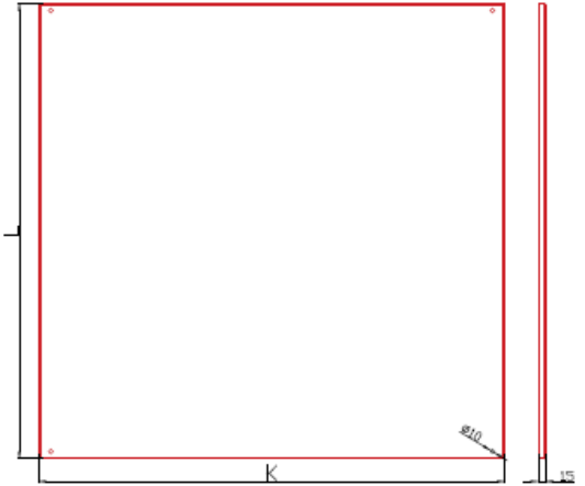
MOUNTING PLATE t=2mm Pre-galvanised Steel
